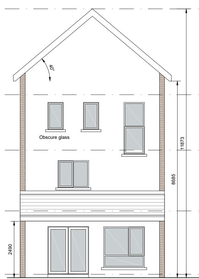
REAR ELEVATION
