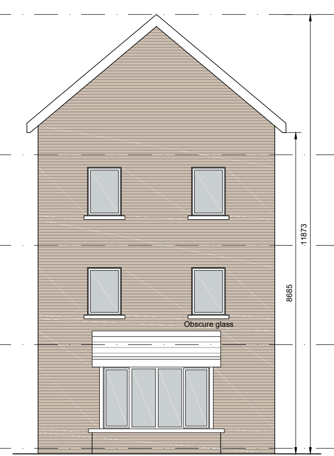
GABLE ELEVATION
