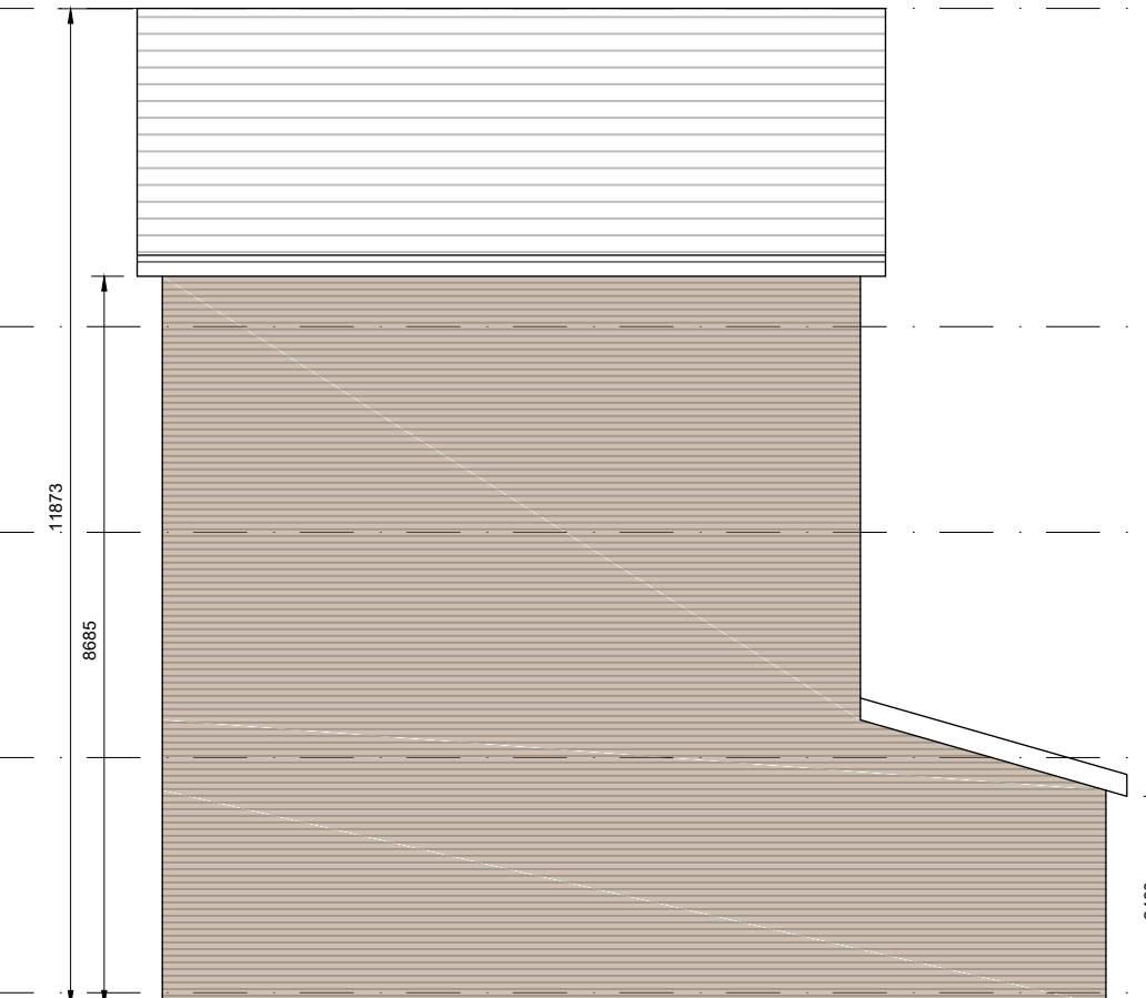
SIDE ELEVATION (north site only)
